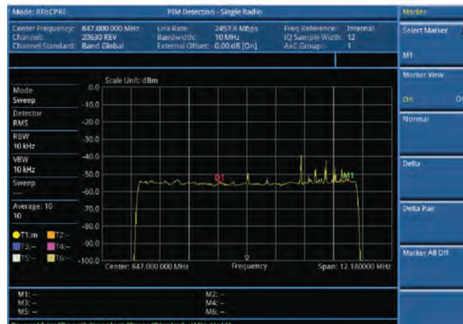
RFoCPRI — Detection - Single Radio
